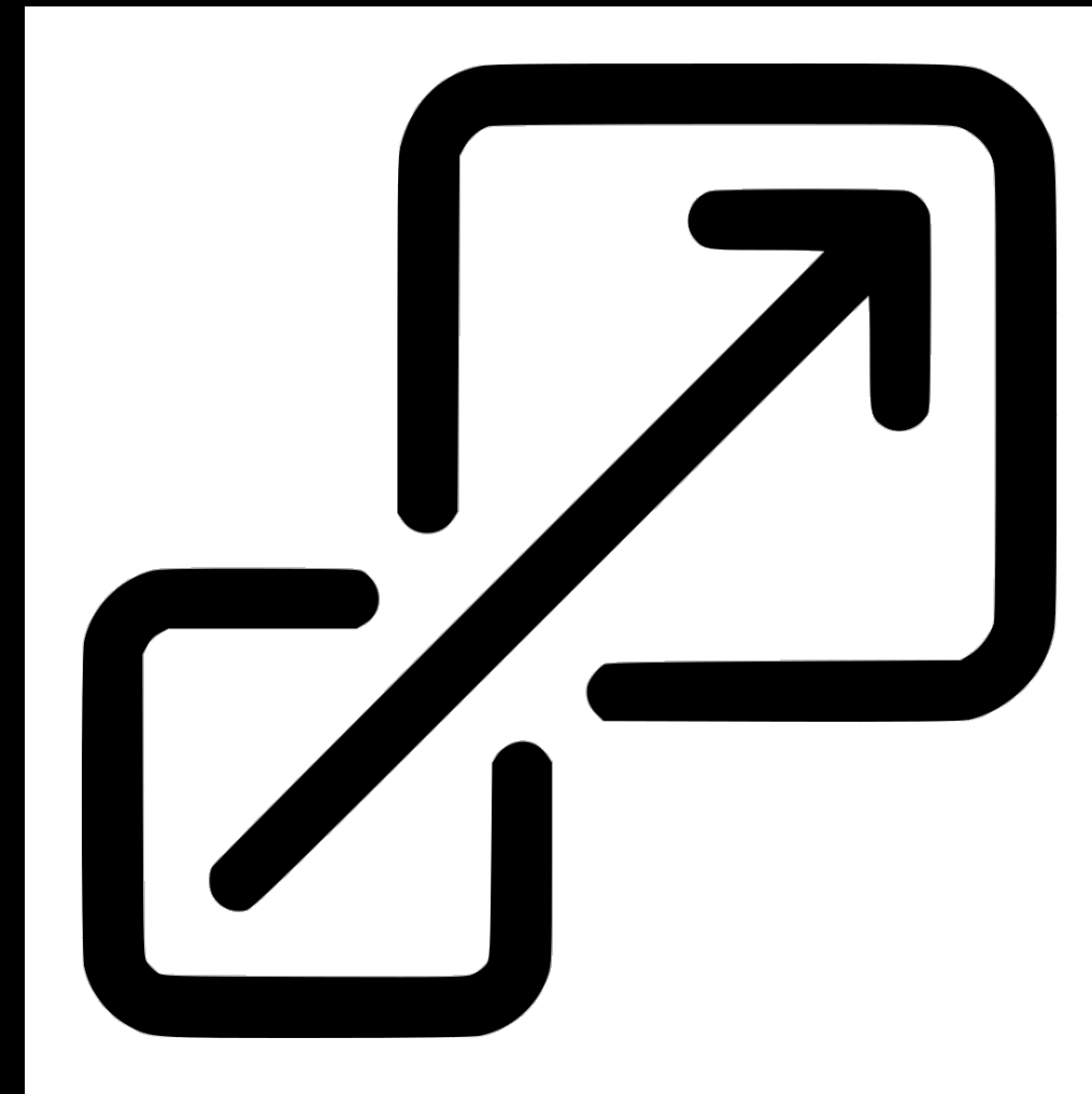
SCALABILITY
